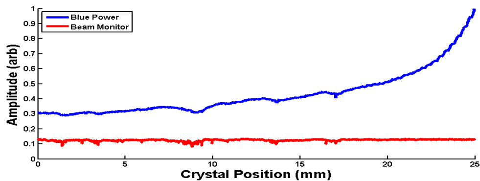
Figure 19. Blue light intensity vs. crystal position
